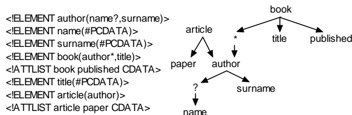
Fig. 5. An example of a DTD graph
