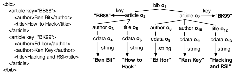
Fig. 4. An example of a Monet tree
