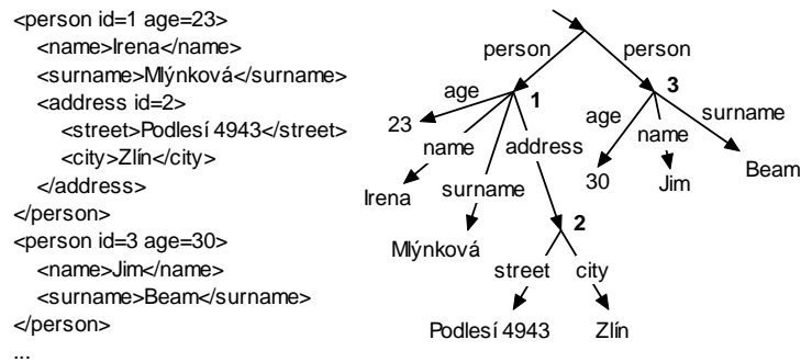
Fig. 1. An example of a generic-tree
