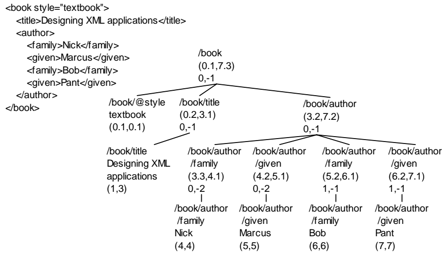
Fig. 3. An example of a simple-path tree
