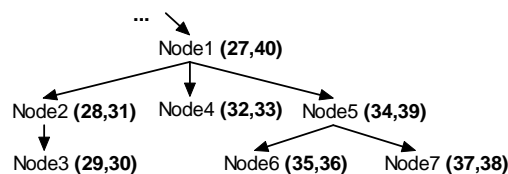
Fig. 2. An example of DF indexing
