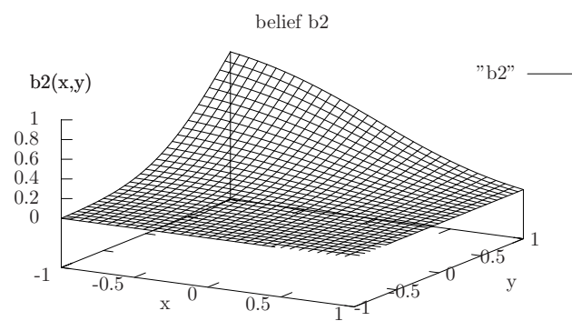
Figure 5.12: Belief function b_2
